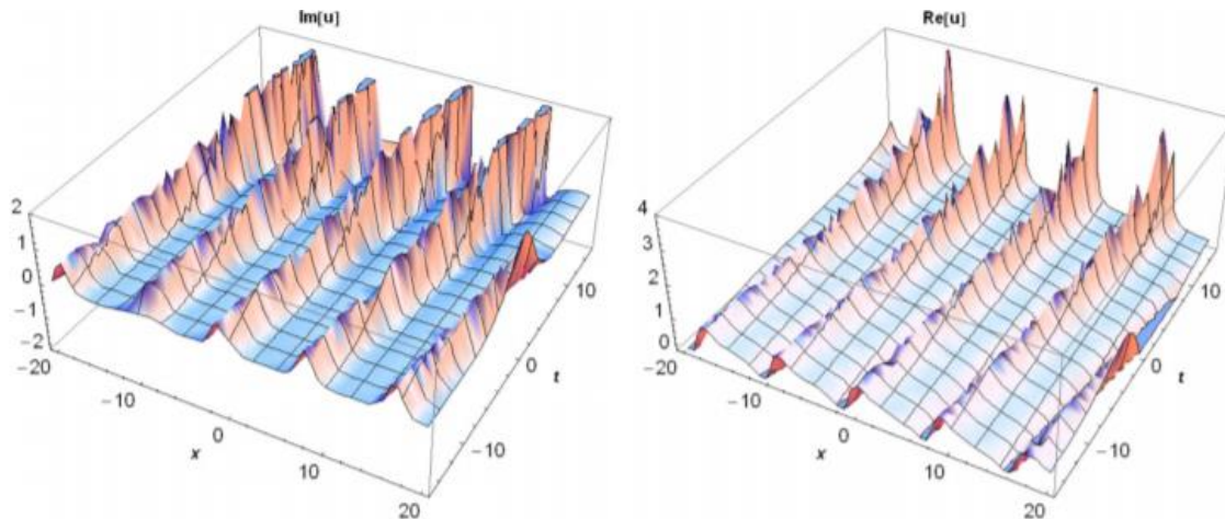
Figure 6: The Three-Dimensional Graphs of Equation (12)
