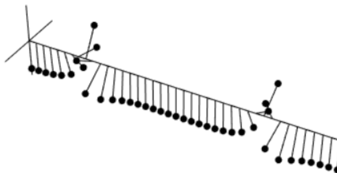
Figure 4: Two Solitons Kink-Kink Collision
