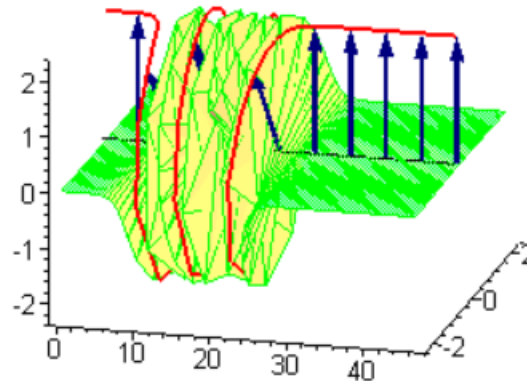
Figure 5: Moving Kink Standing Breather Collision
