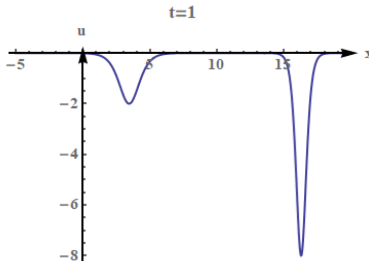
Figure 3: KdV Equation Two Soliton Solution at t = 1
