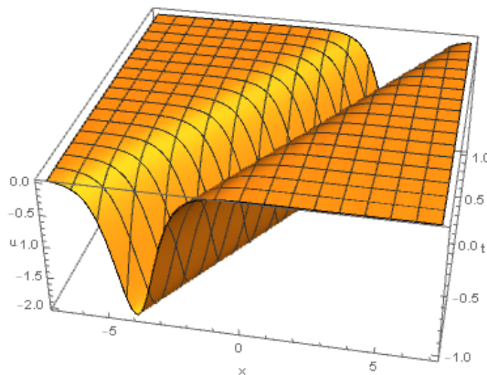
Figure 1: Dark Soliton
