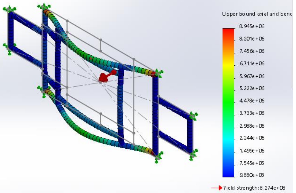
Figure 4: Equivalent Stress for TI-6AL-4V
