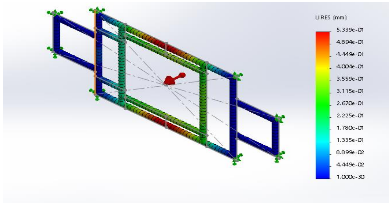
Figure 9: Total Deformation for 304L Steel
