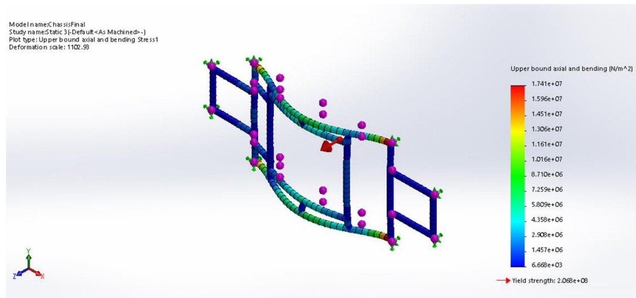
Figure 11: Equivalent Stress for 304L Steel
