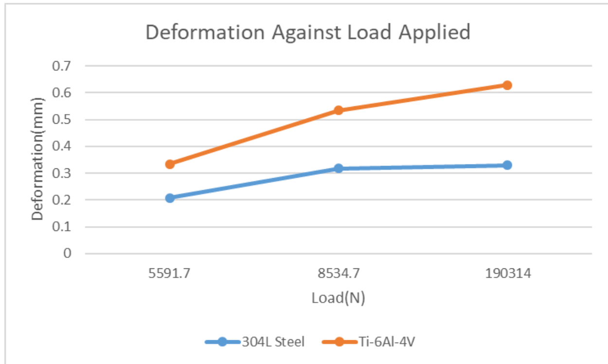
Figure 16: Graph Showing Deformation Against Load Applied
