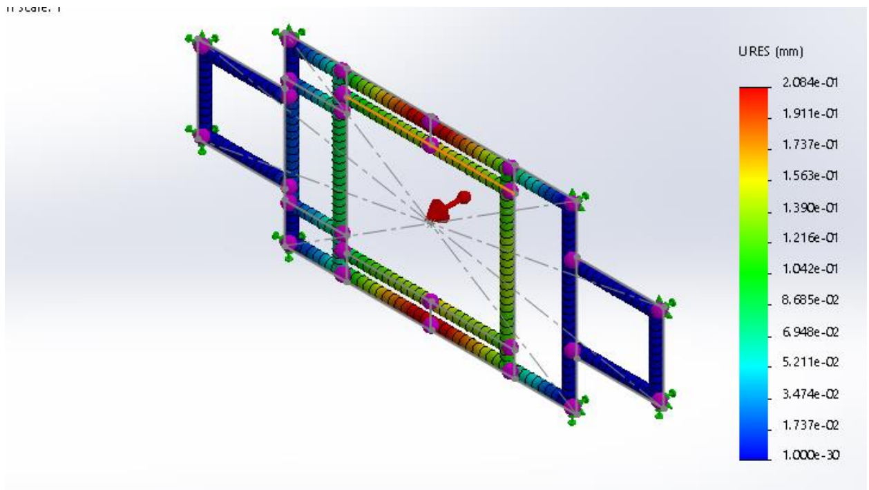
Figure 5: Total Deformation for 304L Steel
