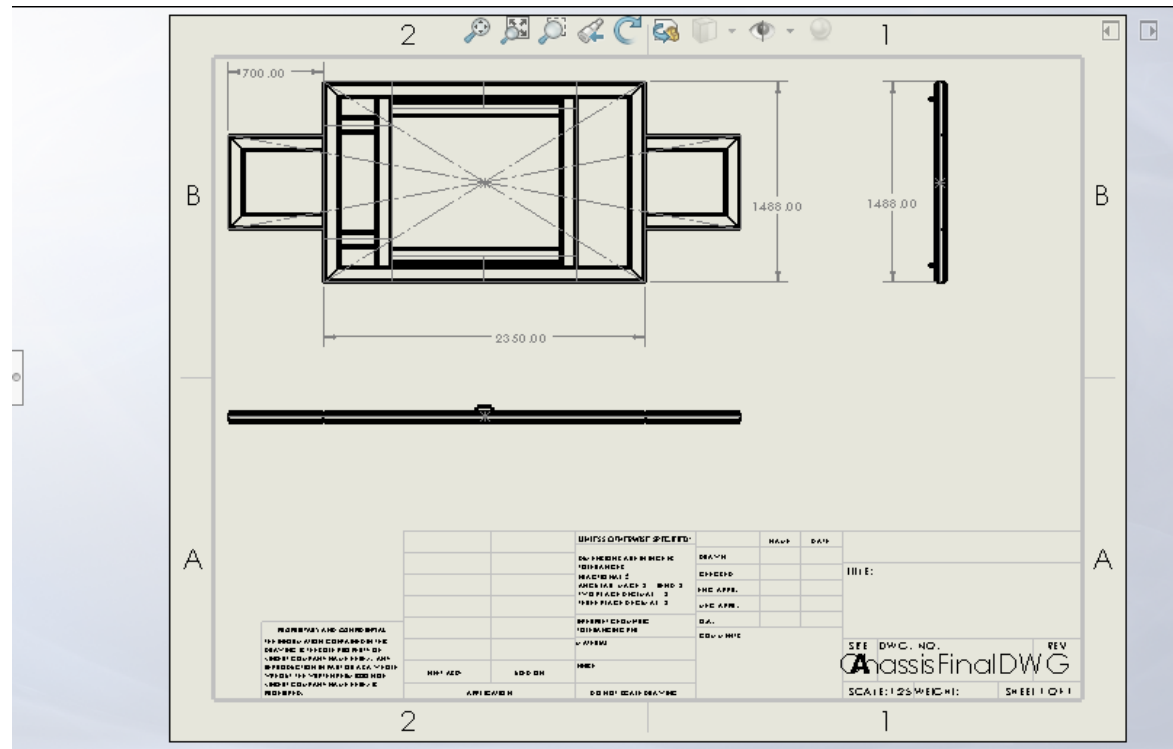
Figure 2: Top, Front, and Side View of the Chassis
