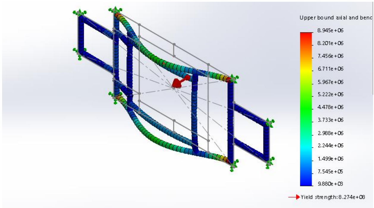
Figure 4: Equivalent Stress for TI-6AL-4V
