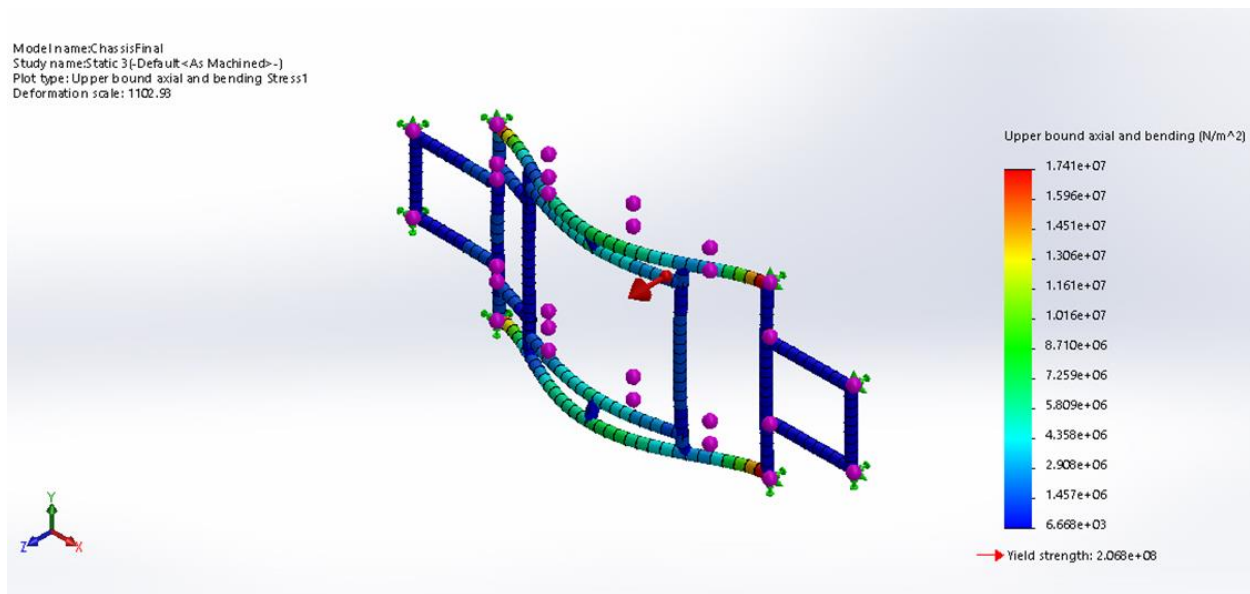
Figure 7: Equivalent Stress for 304L Steel
