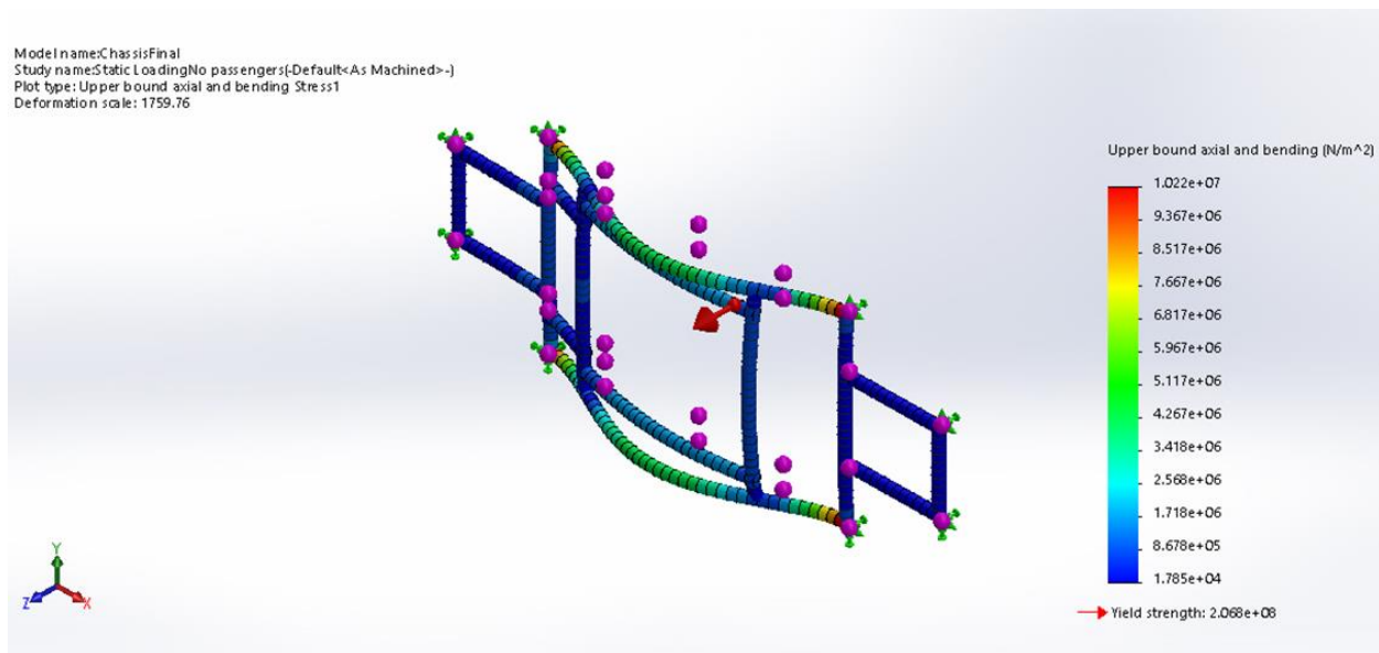
Figure 3: Equivalent Stress for 304L Steel
