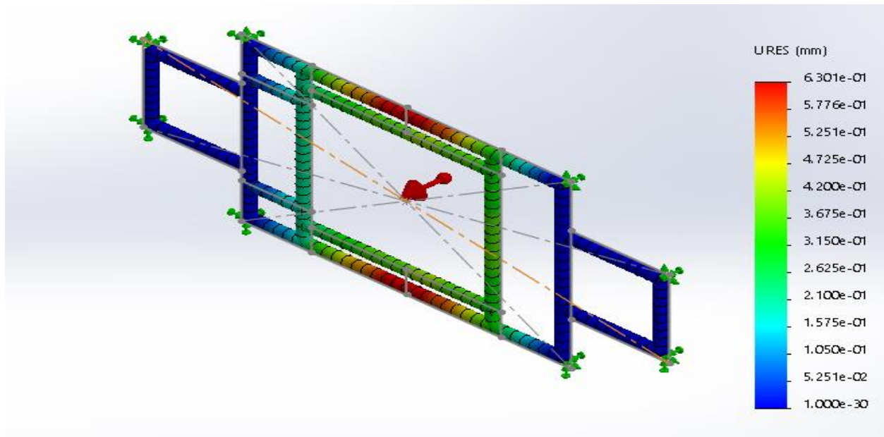
Figure 14: Total Deformation for TI-6AL-4V
