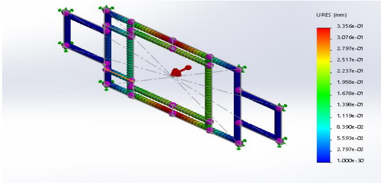
Figure 6: Total Deformation for TI-6AL-4V
