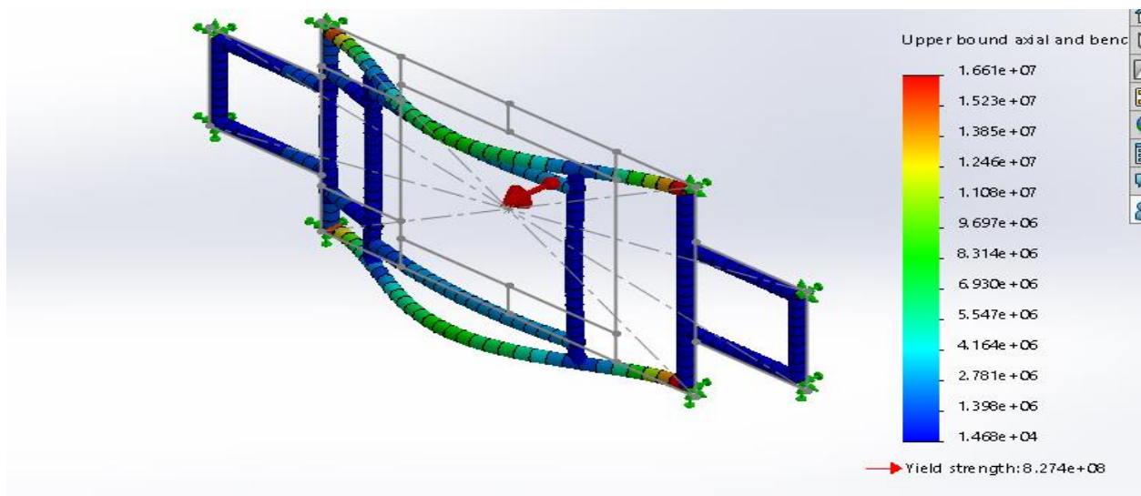
Figure 12: Equivalent Stress for TI-6AL-4V
